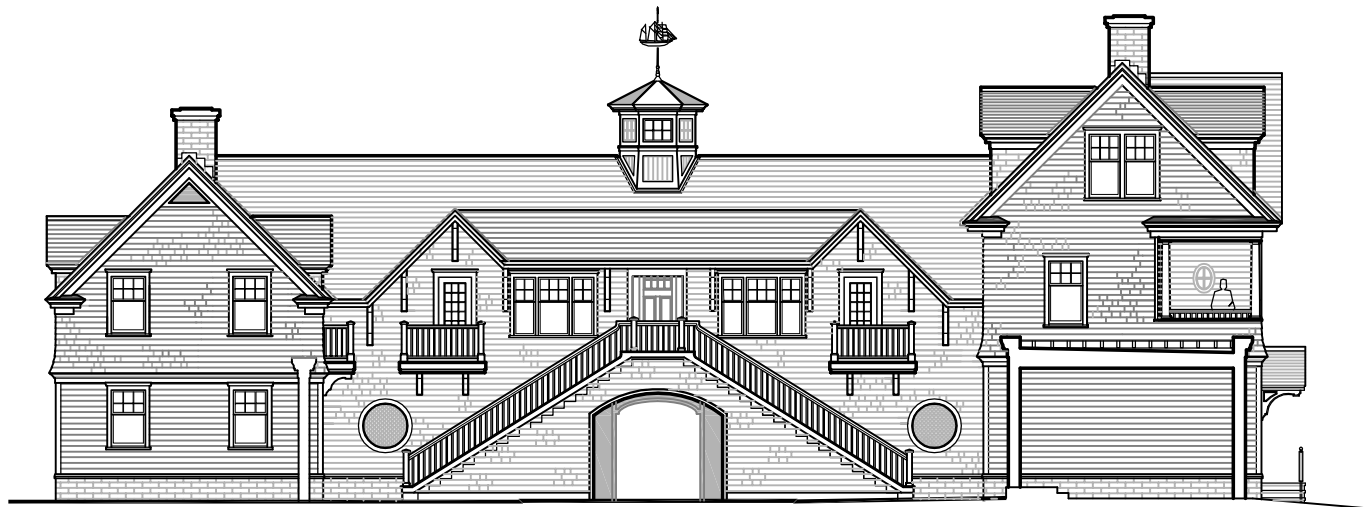
COURTYARD ELEVATION
